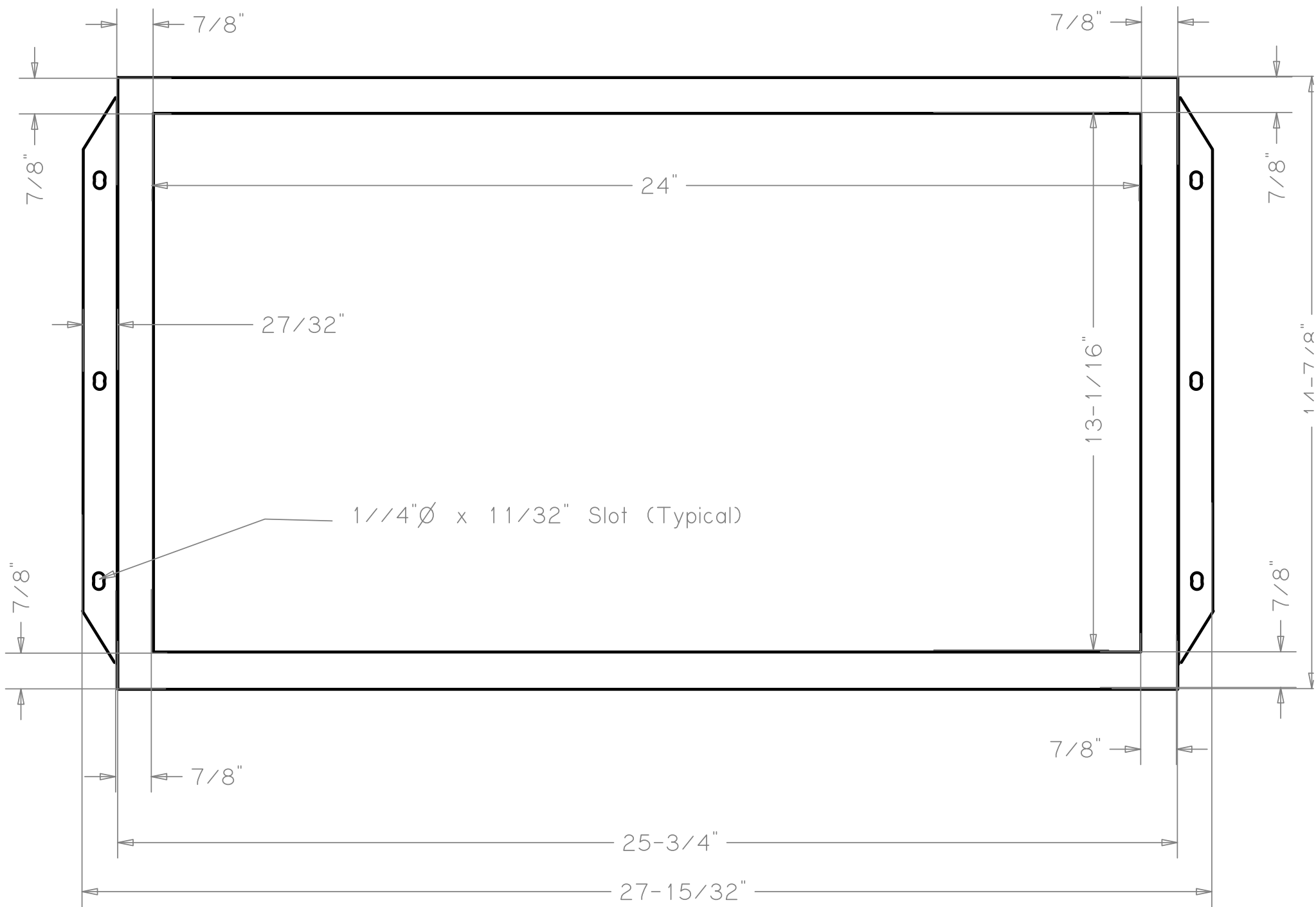
26" Monitor - Top View Holland Computers, Inc. FJM
